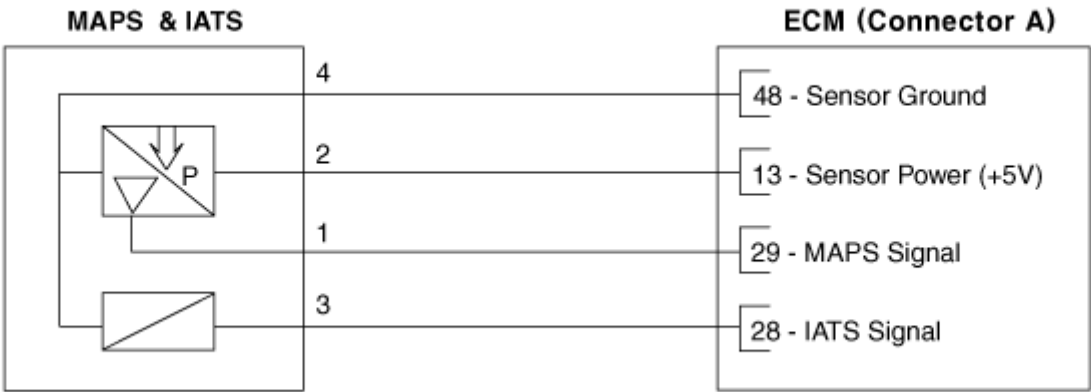
Harness Connector
